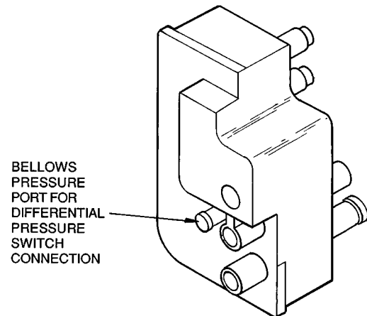
Fig. 74 — Connection for Electric Interlock
